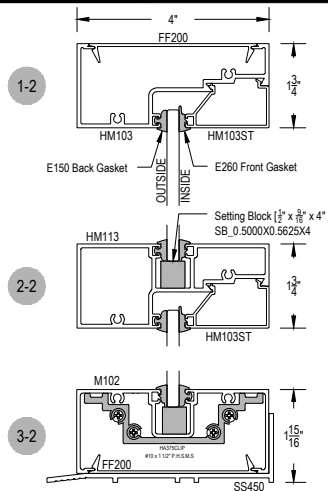
SHEAR BLOCK INSIDE SET
