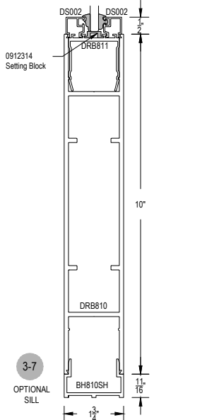
COMPENSATING STICK INSIDE SET
