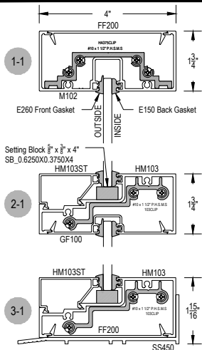
SHEAR BLOCK OUTSIDE SET
