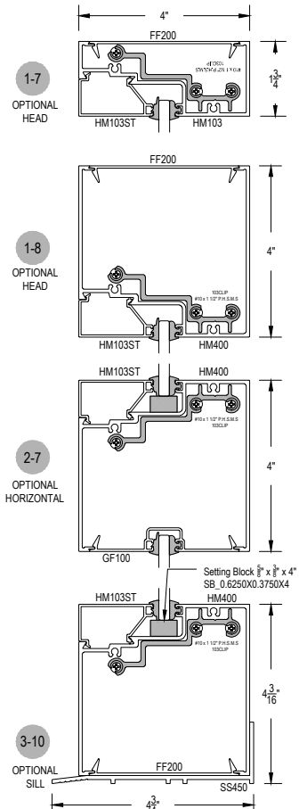
GASKET PLACEMENT FOR INSIDE/OUTSIDE SET SYSTEMS
